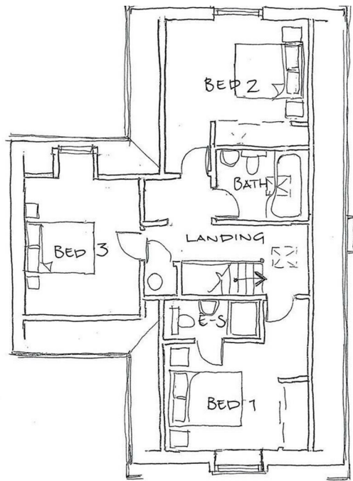
PLOT 2 FIRST FLOOR ~ 1:100
